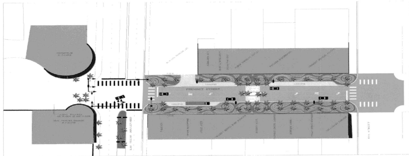
FREMONT STREETSCAPE PREFERRED ALTERNATIVE FROM LAS VEGAS BOULEVARD TO 6TH STREET SCALE: 1" = 20'
