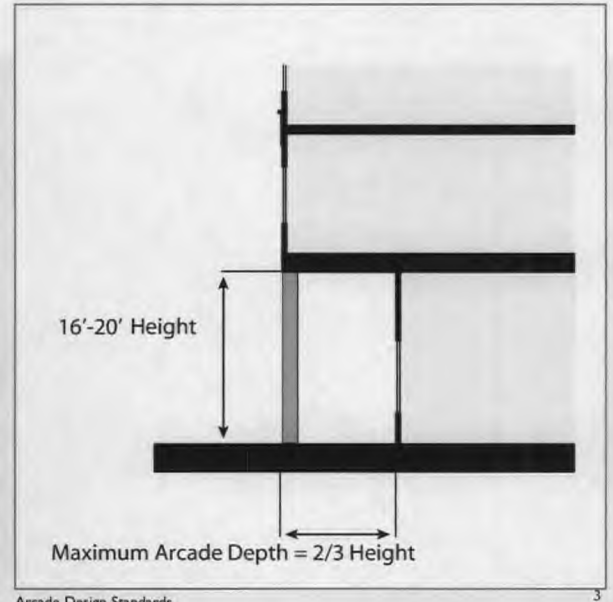
Arcade Design Standards
