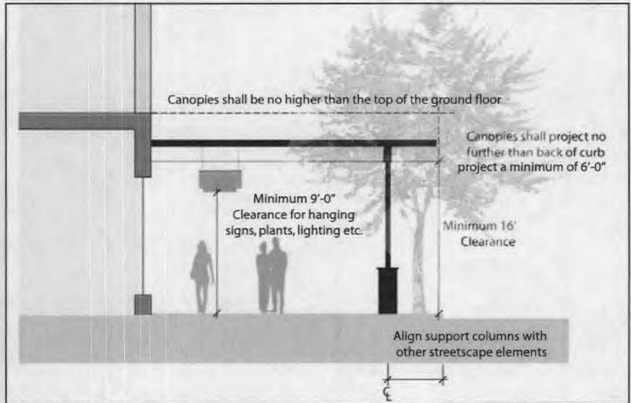
Overhead Canopy and Shading Design Standards
