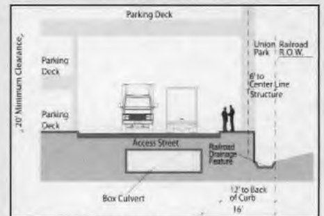
Typical Service Access Section (Along Railroad)
