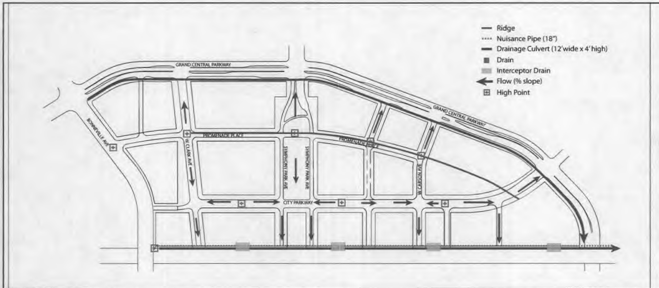
Stormwater Management and Drainage Features
