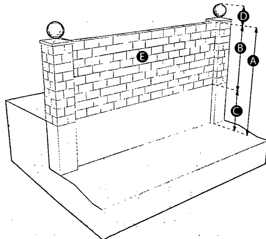
FIGURE 6 - RETAINING AND PERIMETER WALL
