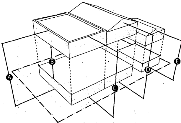
FIGURE 3 - BUILDING HEIGHT
