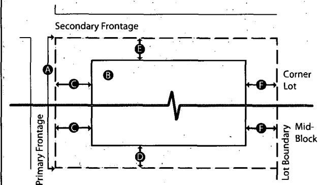
FIGURE 1 - BUILDING PLACEMENT
