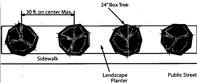
FIGURE 1 - STANDARD PLANTING REQUIREMENT
