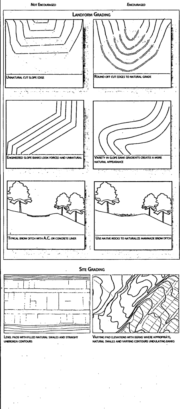
FIGURE 5 - GRADING
