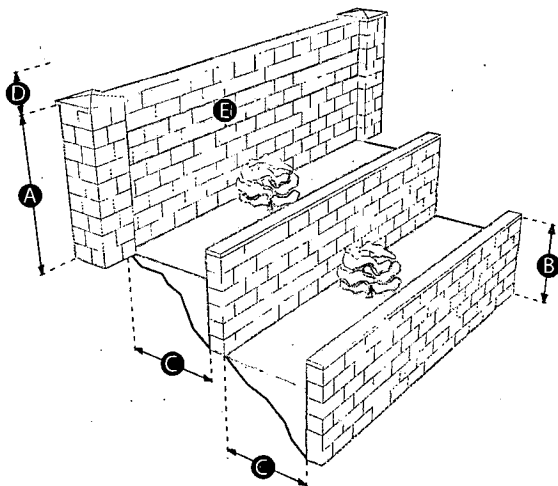
FIGURE 6 - RETAINING AND PERIMETER WALL STANDARD STEPBACK
