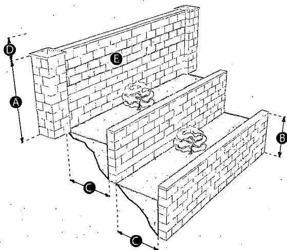
FIGURE 8 - RETAINING AND PERIMETER WALL STANDARD STEPBACK
