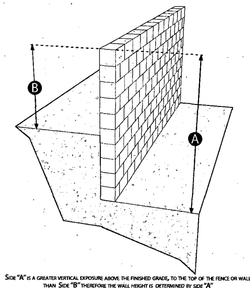
FIGURE 2 - WALL/FENCE HEIGHT MEASUREMENT
