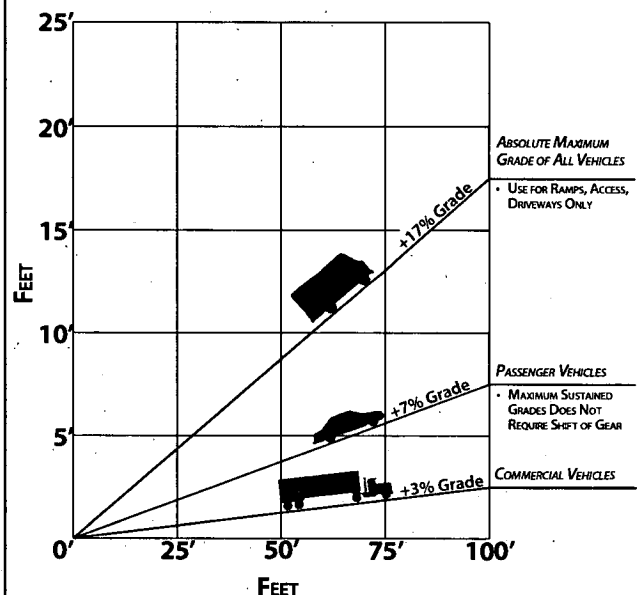
FIGURE 11- ROADWAY MAXIMUM SLOPE COMPARISON
