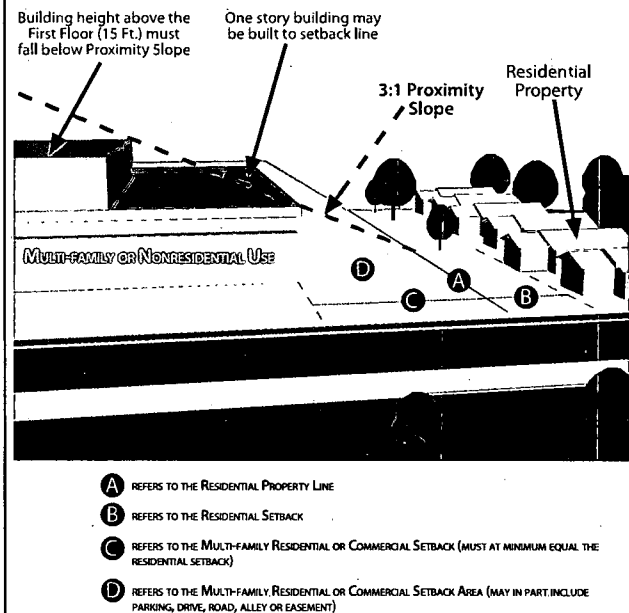
FIGURE 4 - PROXIMITY SLOPE - 3:1 SLOPE REQUIREMENT
