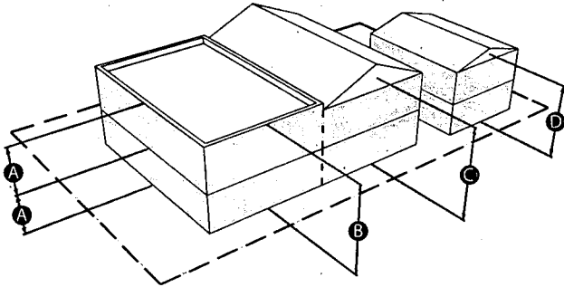
FIGURE 3 - BUILDING HEIGHT
