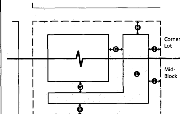
FIGURE 2 - ACCESSORY STRUCTURES
