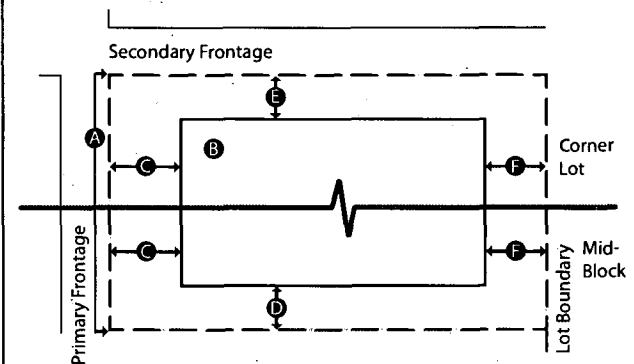
FIGURE 1 - BUILDING PLACEMENT
