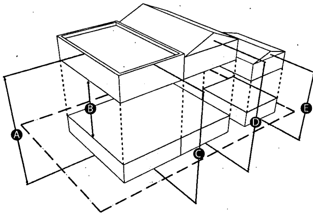
FIGURE 3 - BUILDING HEIGHT
