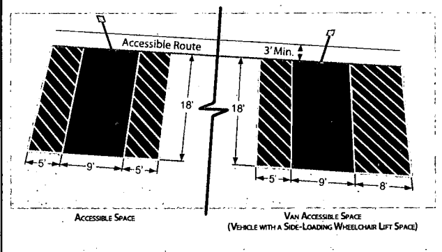
FIGURE 2 - HANDICAPPED PARKING DIMENSIONS
