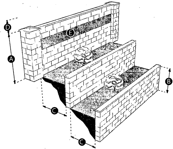
FIGURE 9 - RETAINING AND PERIMETER WALL STANDARD STEPBACK
