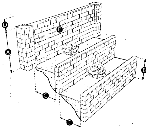
FIGURE 7 - RETAINING AND PERIMETER WALL STANDARD STEPBACK
