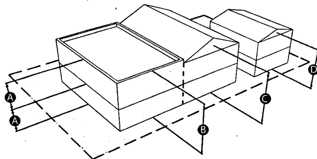
FIGURE 4 - BUILDING HEIGHT
