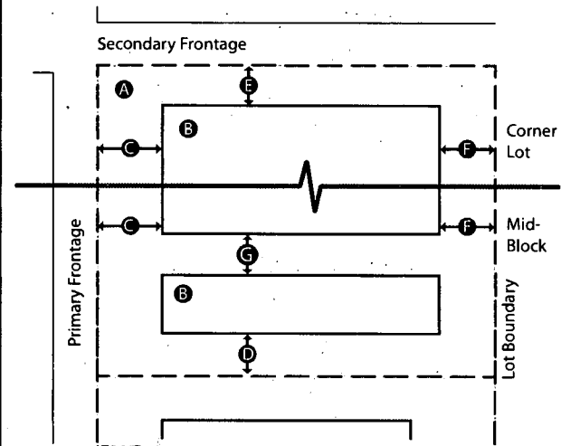
FIGURE 1 - BUILDING PLACEMENT
