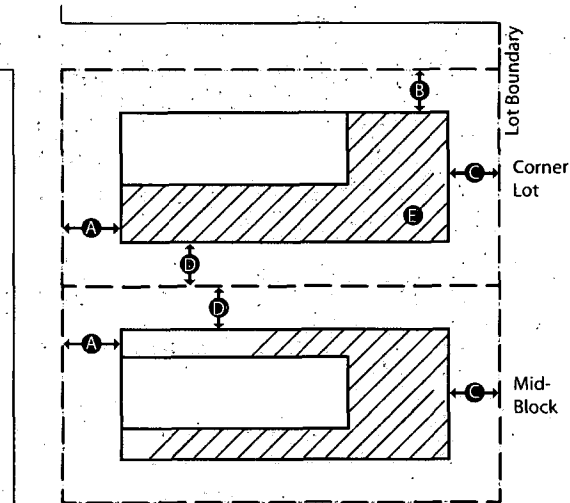
FIGURE 2 - ACCESSORY STRUCTURES
