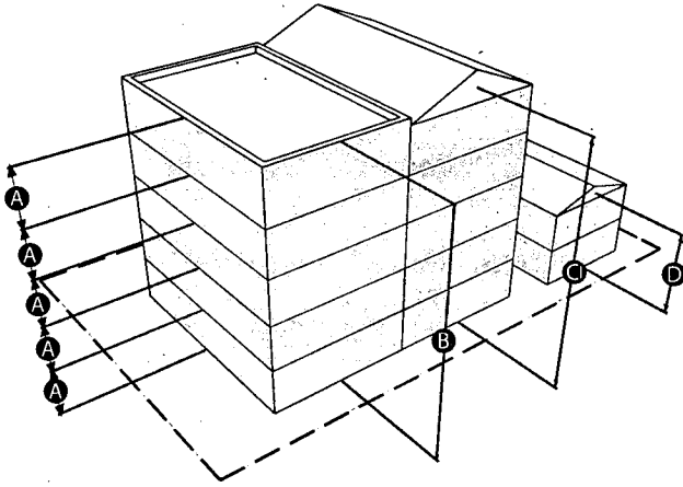
FIGURE 3 - BUILDING HEIGHT
