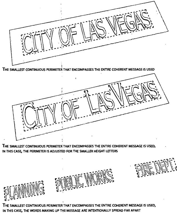
FIGURE 11 - SIGN AREA MEASUREMENT - CHANNEL LETTERS
