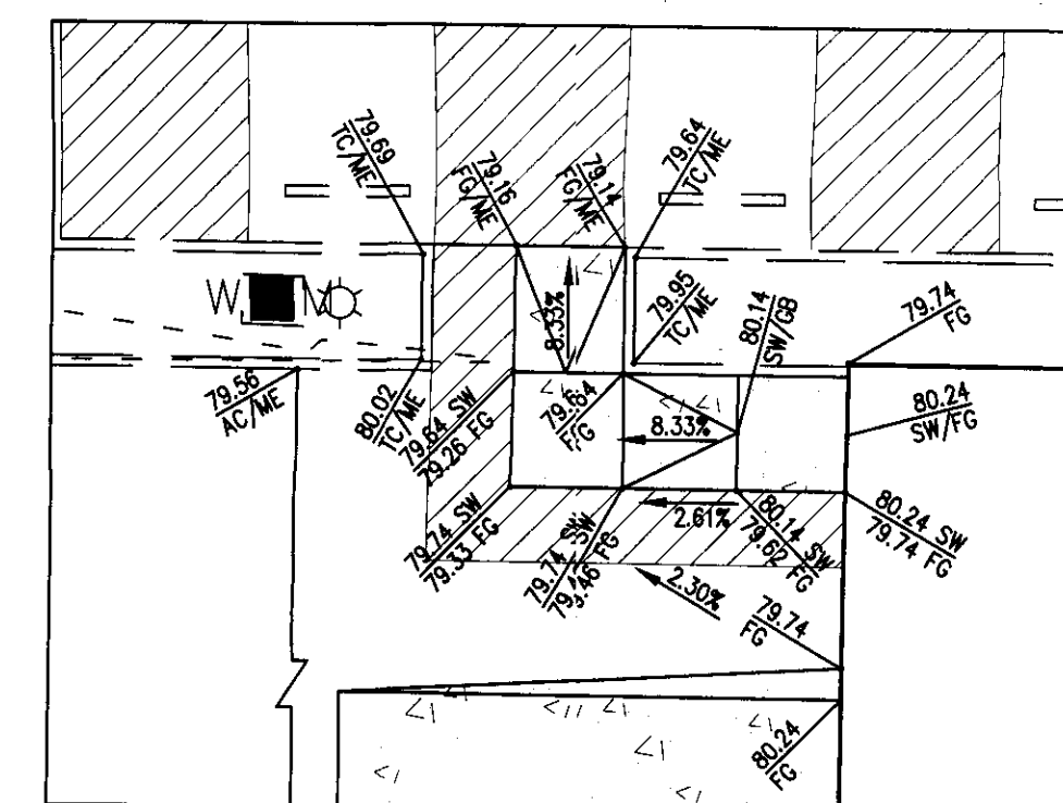
ENLARGED VIEW "B" SCALE 1"=10'
