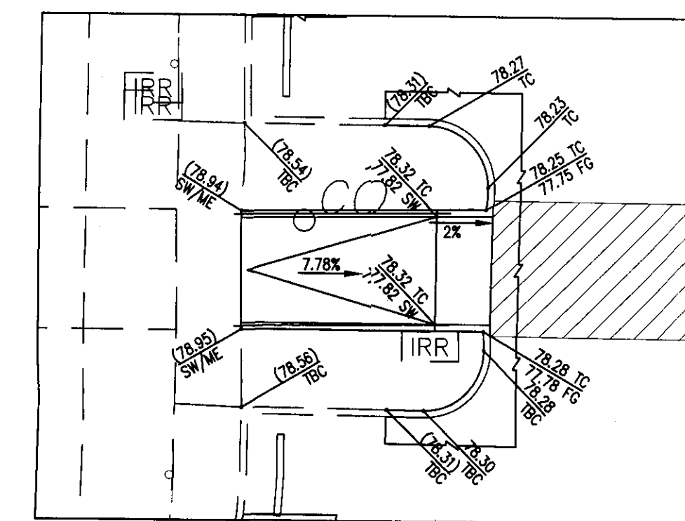
ENLARGED VIEW "A" SCALE 1"=10'
