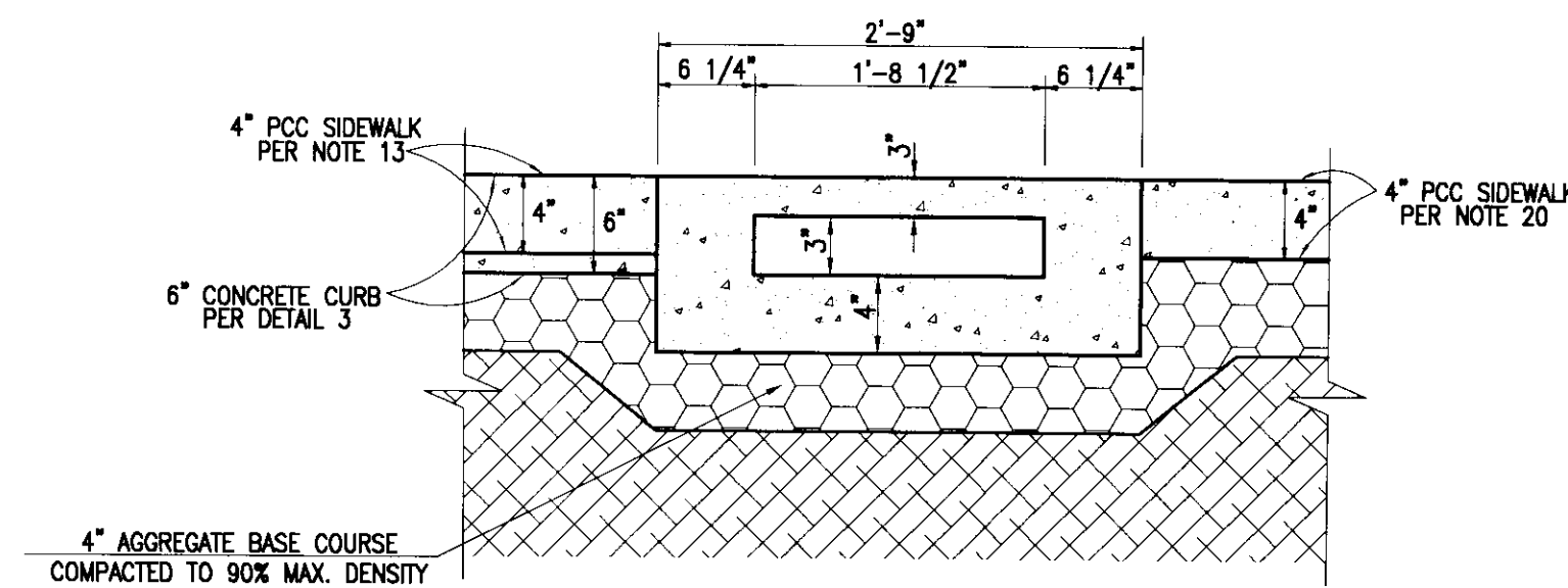
2.0' WIDE BOX UNDER SIDEWALK ⑥ N.T.S.
