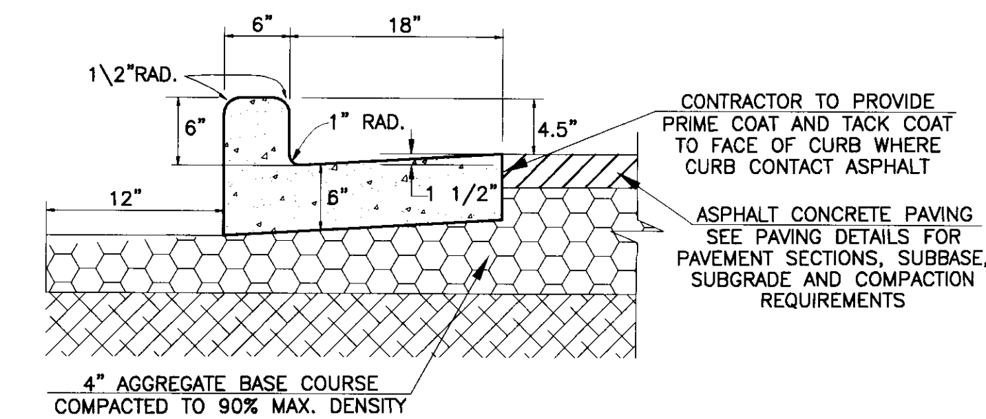
6' CURB AND GUTTER DETAIL: ④ N.T.S.
