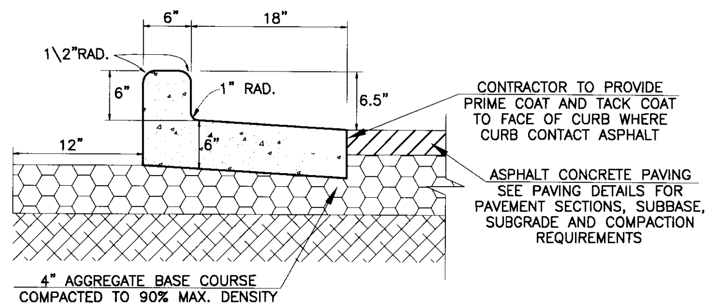
6' CONCRETE CURB ONLY DETAIL: ③ N.T.S.
