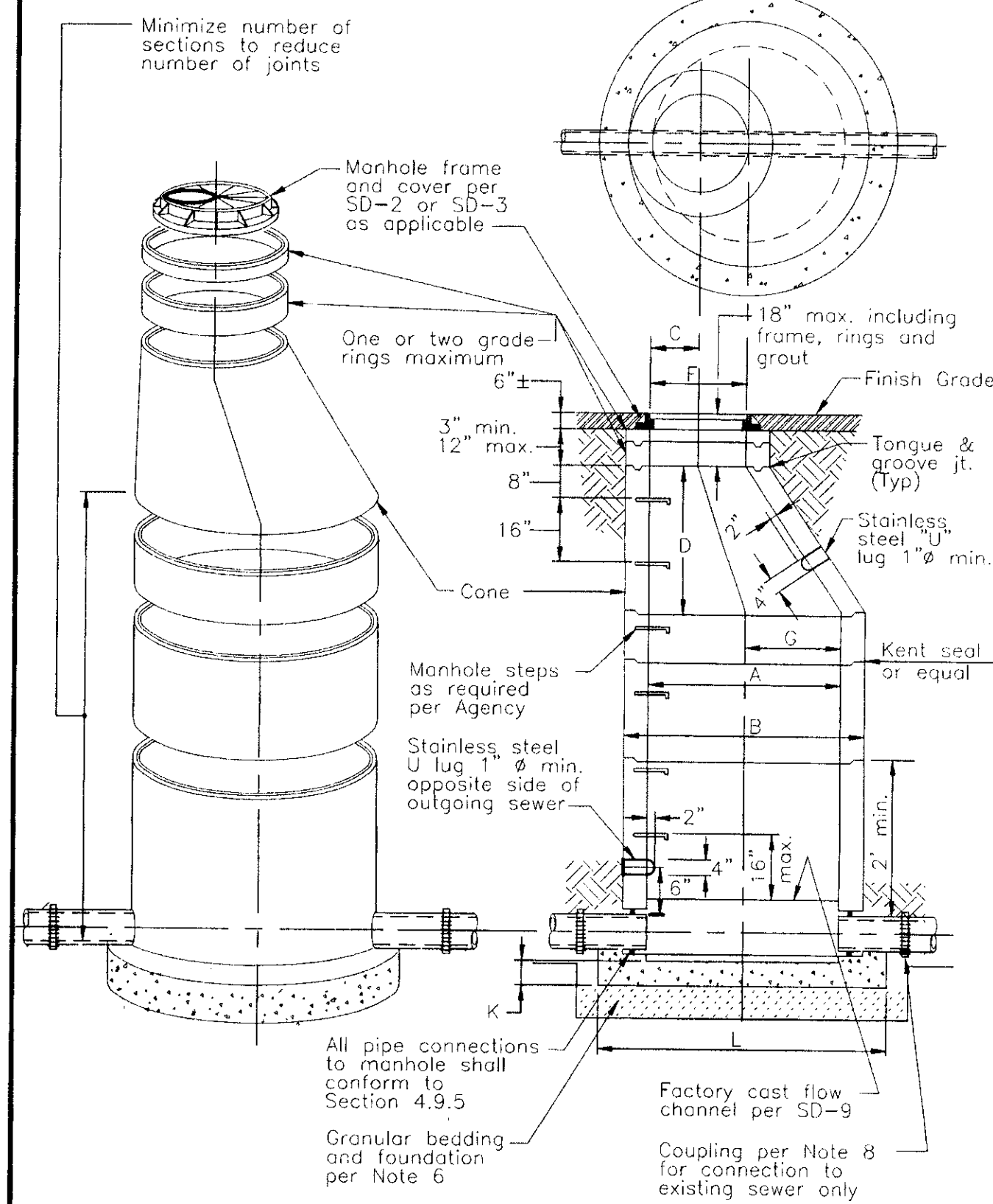
STANDARD PRE-CAST MANHOLE
