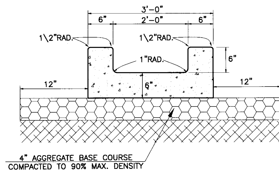
24' CONCRETE CHANNEL DETAIL: ⑤ N.T.S.
