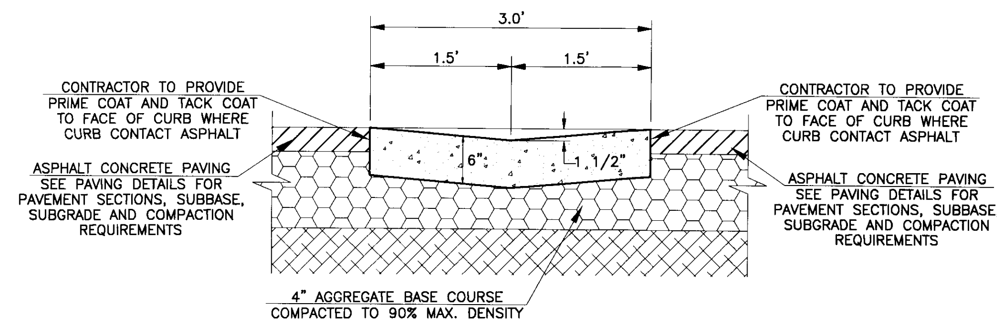
3' WIDE CONCRETE VALLEY GUTTER: ⑦ N.T.S.
