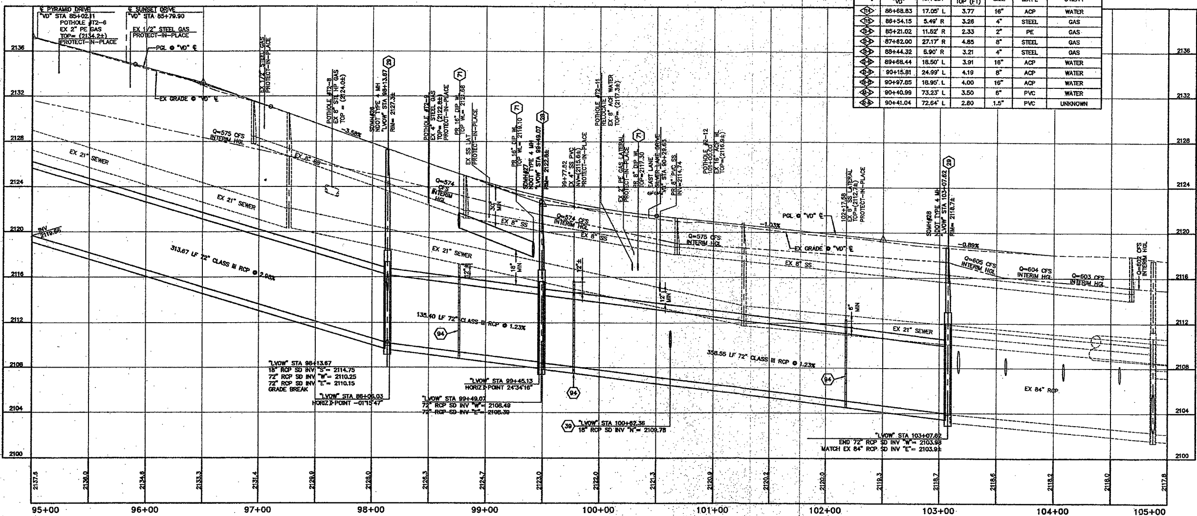
PROFILE - STORM DRAIN CENTERLINE ALIGNMENT "LVOW"
