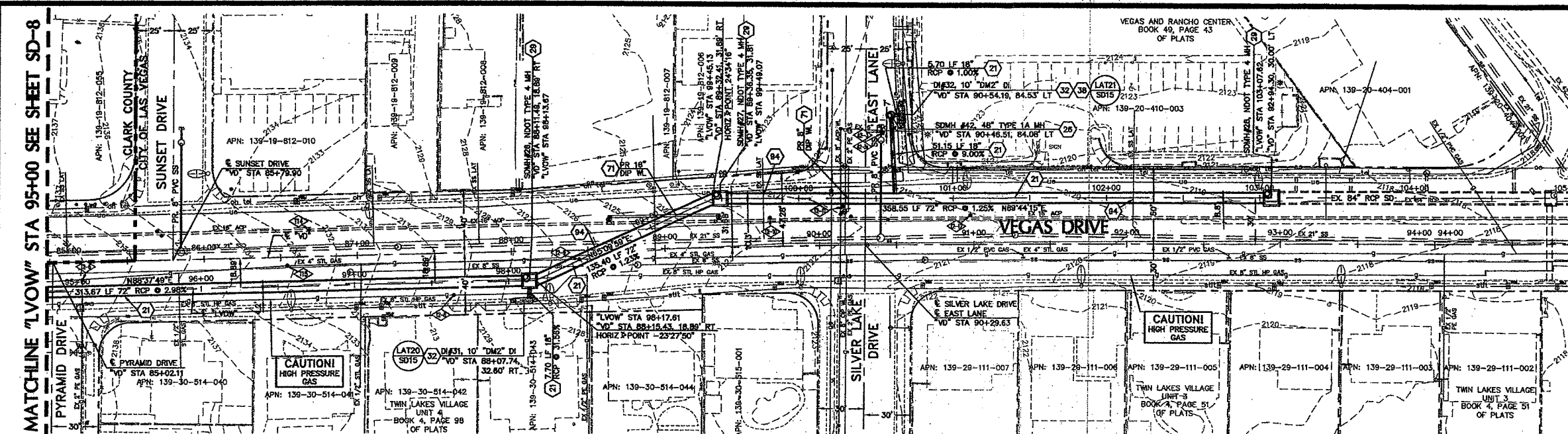
PLAN-STORM DRAIN CENTERLINE ALIGNMENT "LVOW"
