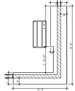
2 PLAN DTL @ PASS THRU
