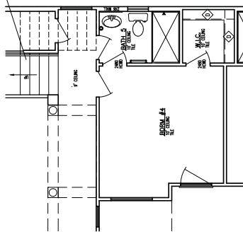
(2) BDRM #4 OPT. SCALE: 1/4" = 1'-0"
