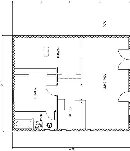
1 EXISTING BLDG C 1ST FLOOR PLAN (NOT USED) 1/4" = 1'-0"
