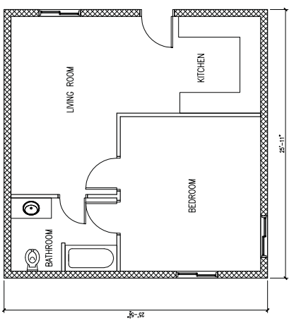
1 EXISTING BLDG C 1ST FLOOR PLAN (NOT USED) 1/4" = 1'-0"
