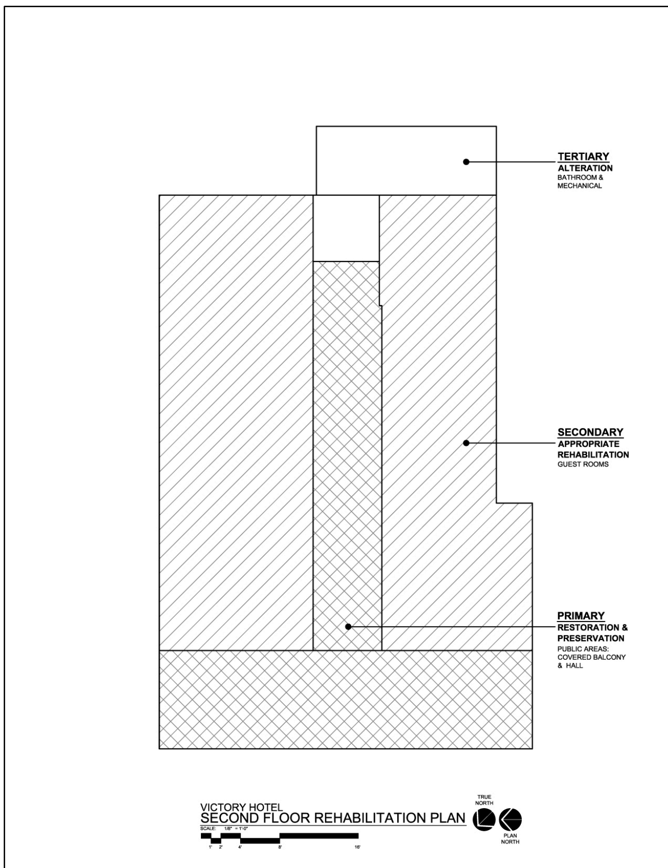
Figure 18. Second floor rehabilitation plan.
