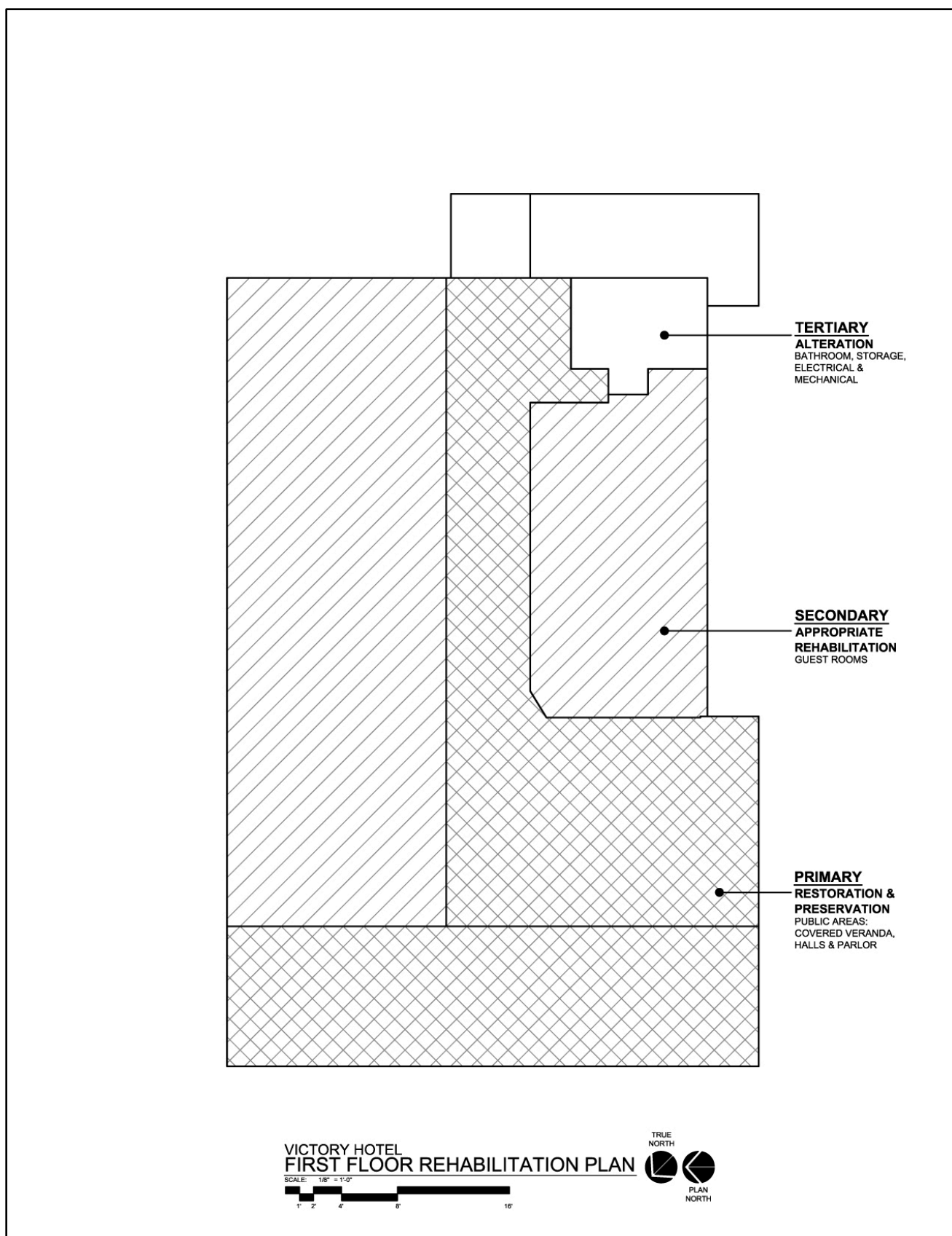
Figure 17. First floor rehabilitation plan.
