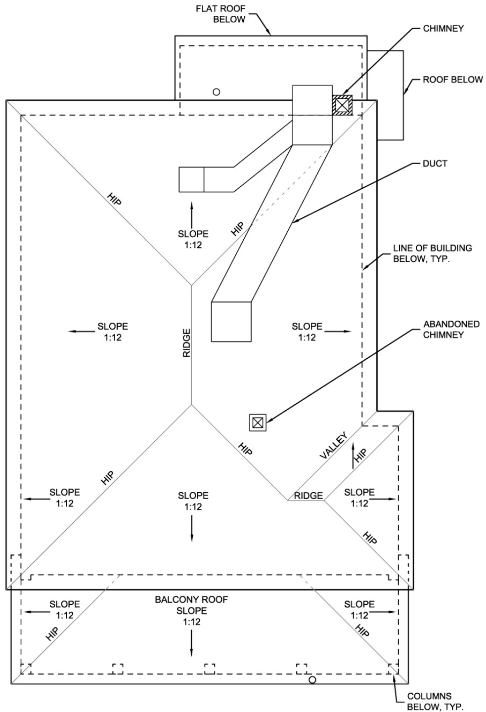
VICTORY HOTEL ROOF PLAN
