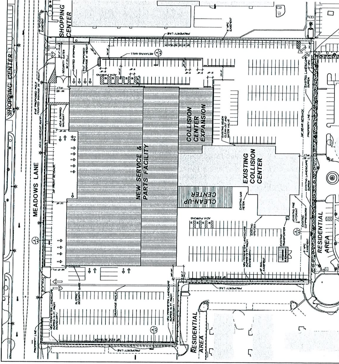
1 SITE PLAN
