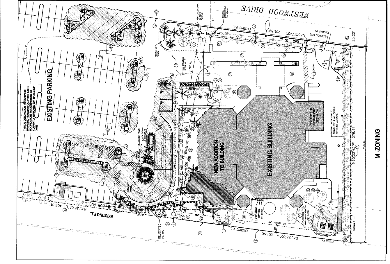
2 LANDSCAPE PLAN
