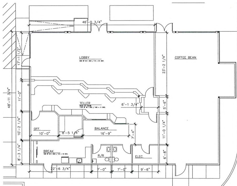
FLOOR PLAN 3/16" = 1' - 0"
