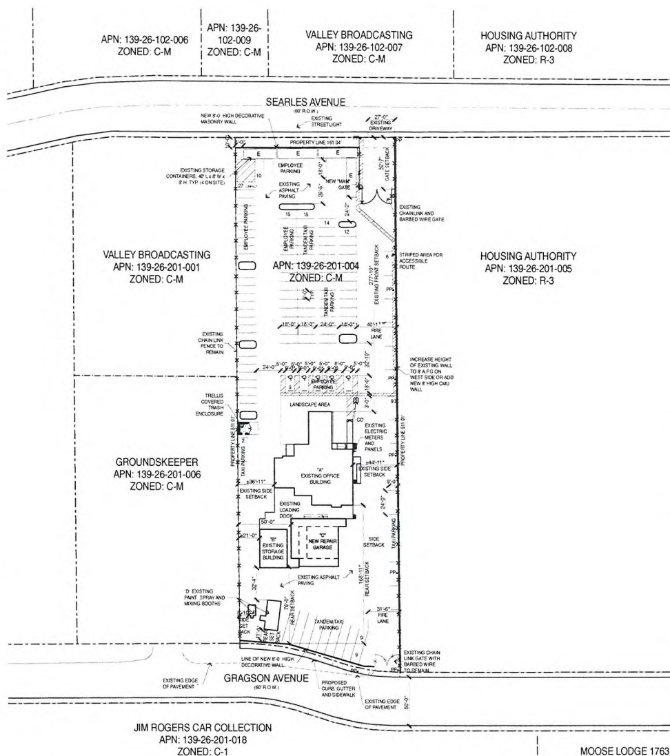
SITE PLAN 1" = 40'
