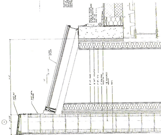
SKYLIGHT SECTION AT PARAPET
