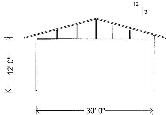
END ELAVATION
