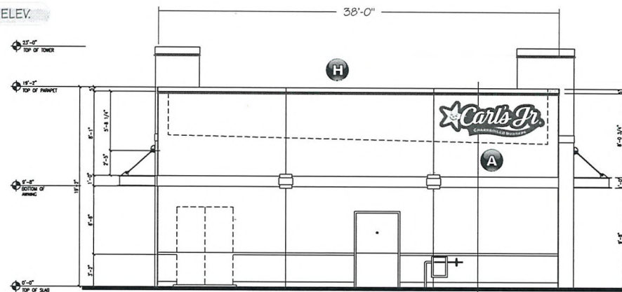
PROPOSED ELEV.
