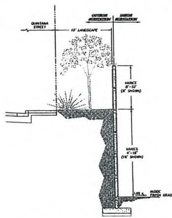
RETAINING WALL ALONG QUINTANA STREET SECTION VIEW
