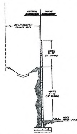
RETAINING WALL ALONG WESTERN BOUNDARY SECTION VIEW
