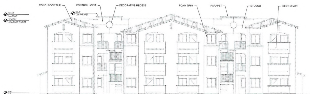
Rear Elevation
