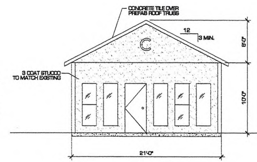
WEST ELEVATION SCALE: 1/4" = 1'-0"
