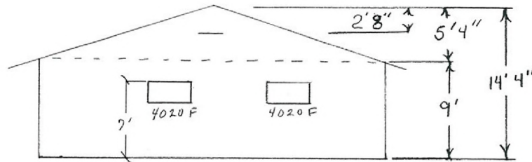
LEFT ELEVATION (WEST)
