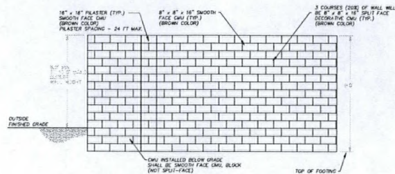
BLOCK WALL DETAIL
