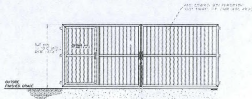
DOUBLE SWING GATE ELEVATION
