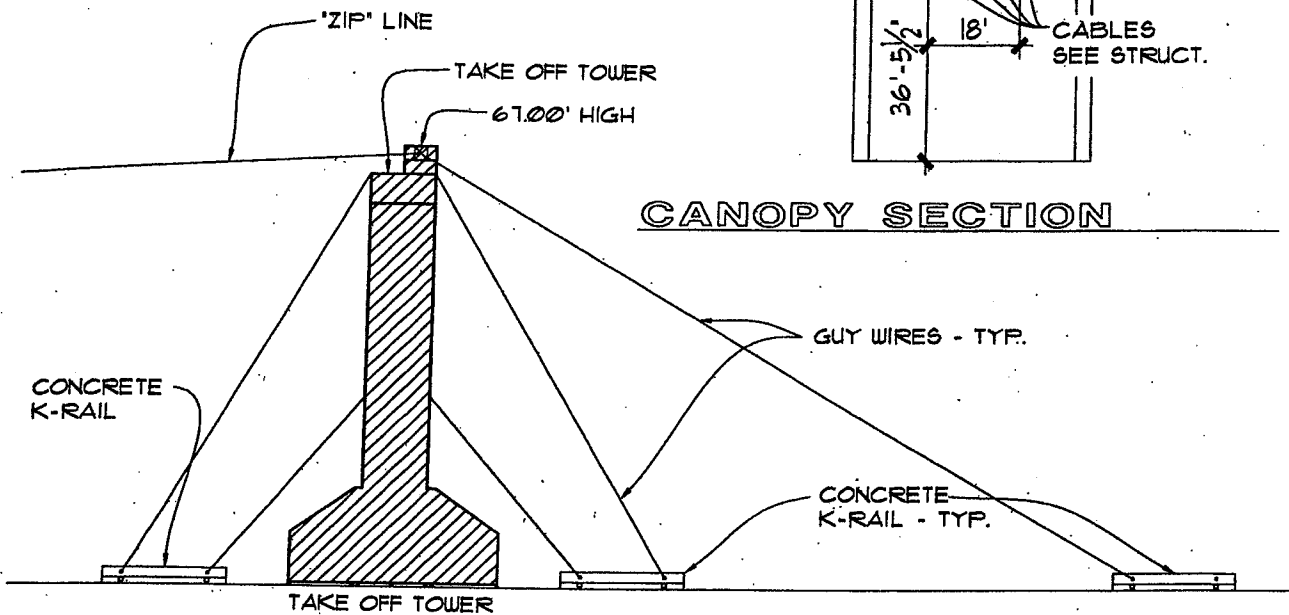
TAKE OFF TOWER ELEVATION
