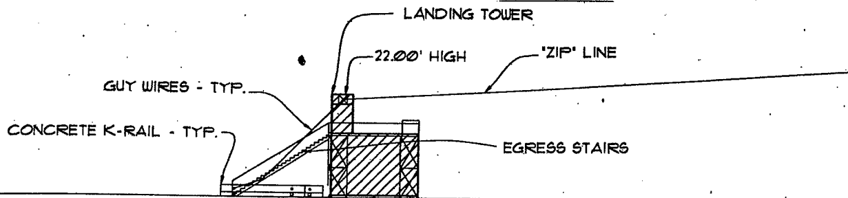
LANDING TOWER ELEVATION
