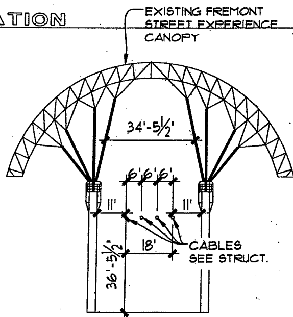
CANOPY SECTION
