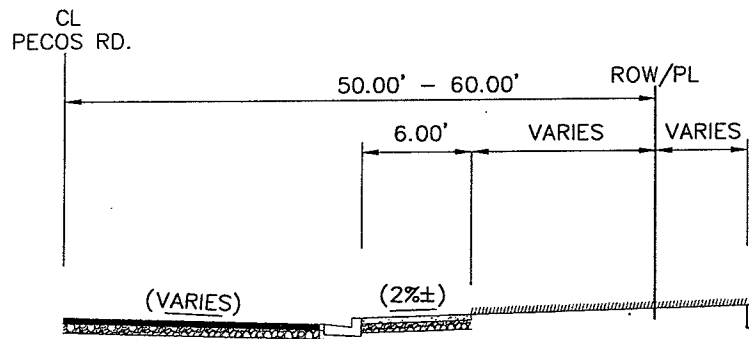
TYPICAL SECTION PECOS RD NTS
