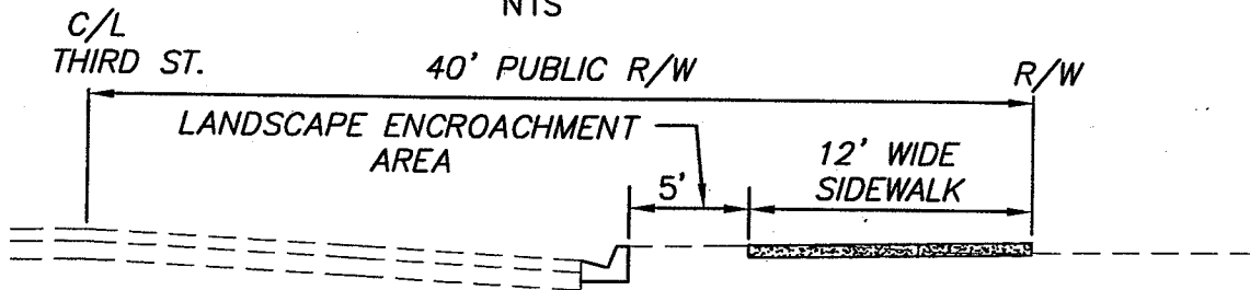
SECTION "A" NTS
