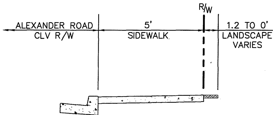
ALEXANDER ROAD SECTION N.T.S.
