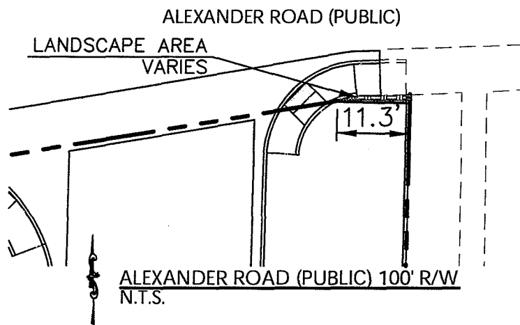
ALEXANDER ROAD SECTION N.T.S.
