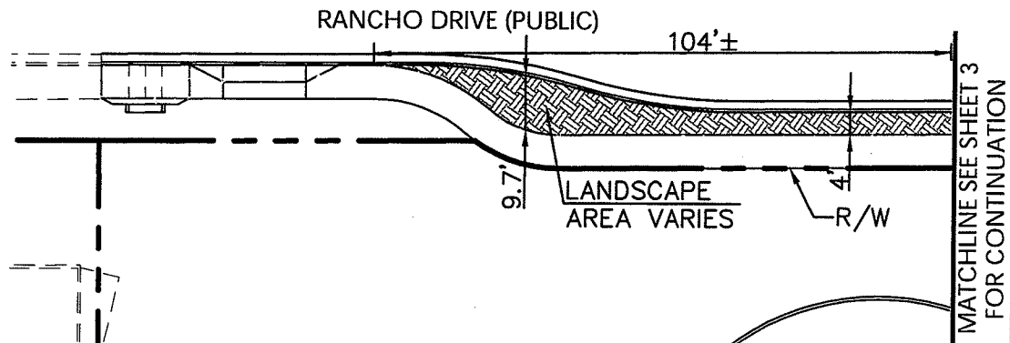
RANCHO DRIVE (PUBLIC) 142.5 NDOT' R/W N.T.S.
