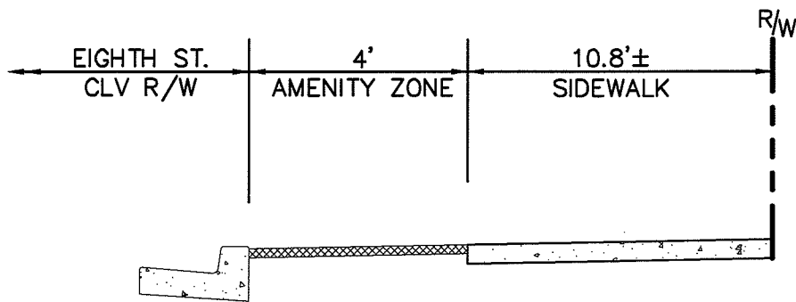
EIGHTH STREET SECTION N.T.S.
