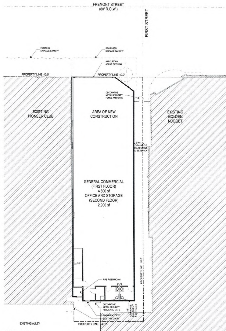
SITE PLAN
