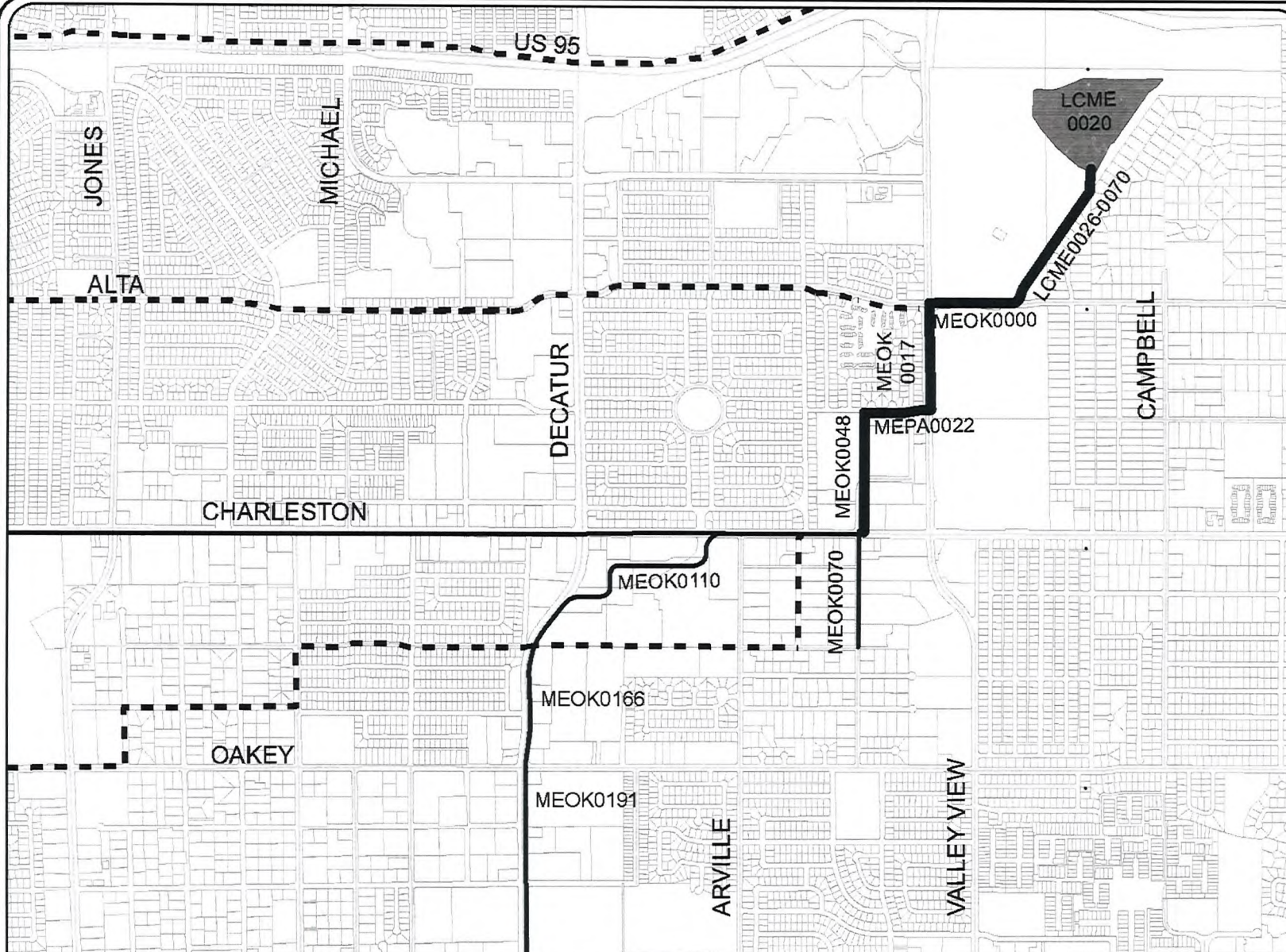
EXHIBIT A OAKEY - MEADOWS STORM DRAIN, PHASE I
