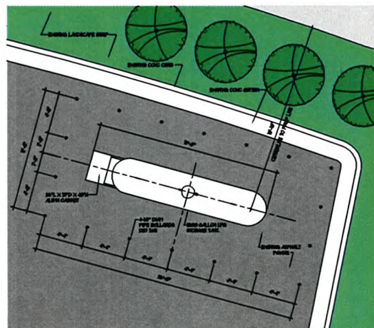
ENLARGED PLAN
