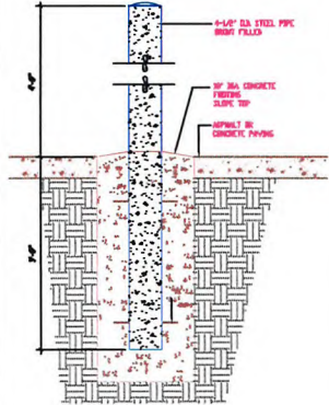
PIPE BOLLARD
