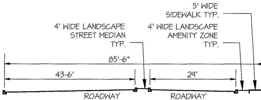
SECTION F-F AMENITY ZONE
