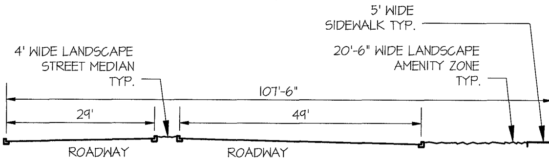
SECTION D-D AMENITY ZONE TYP.
