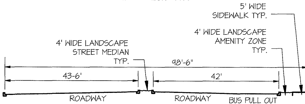
SECTION E-E AMENITY ZONE W/BUS PULLOUT TYP.
