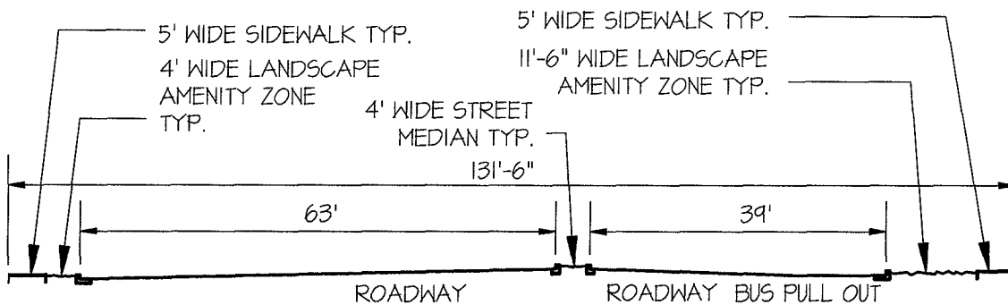
SECTION B-B AMENITY ZONE TYP.
