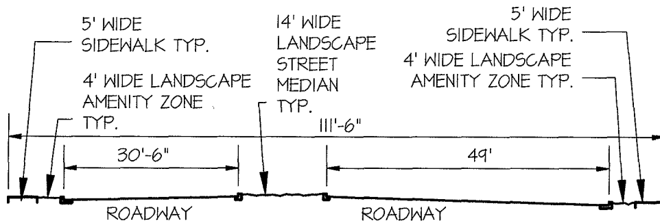
SECTION A-A AMENITY ZONE TYP.
