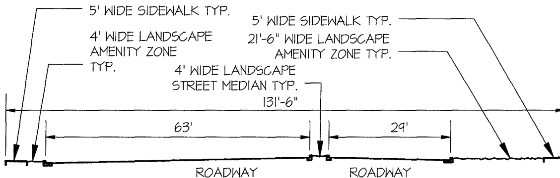
SECTION C-C AMENITY ZONE TYP.
