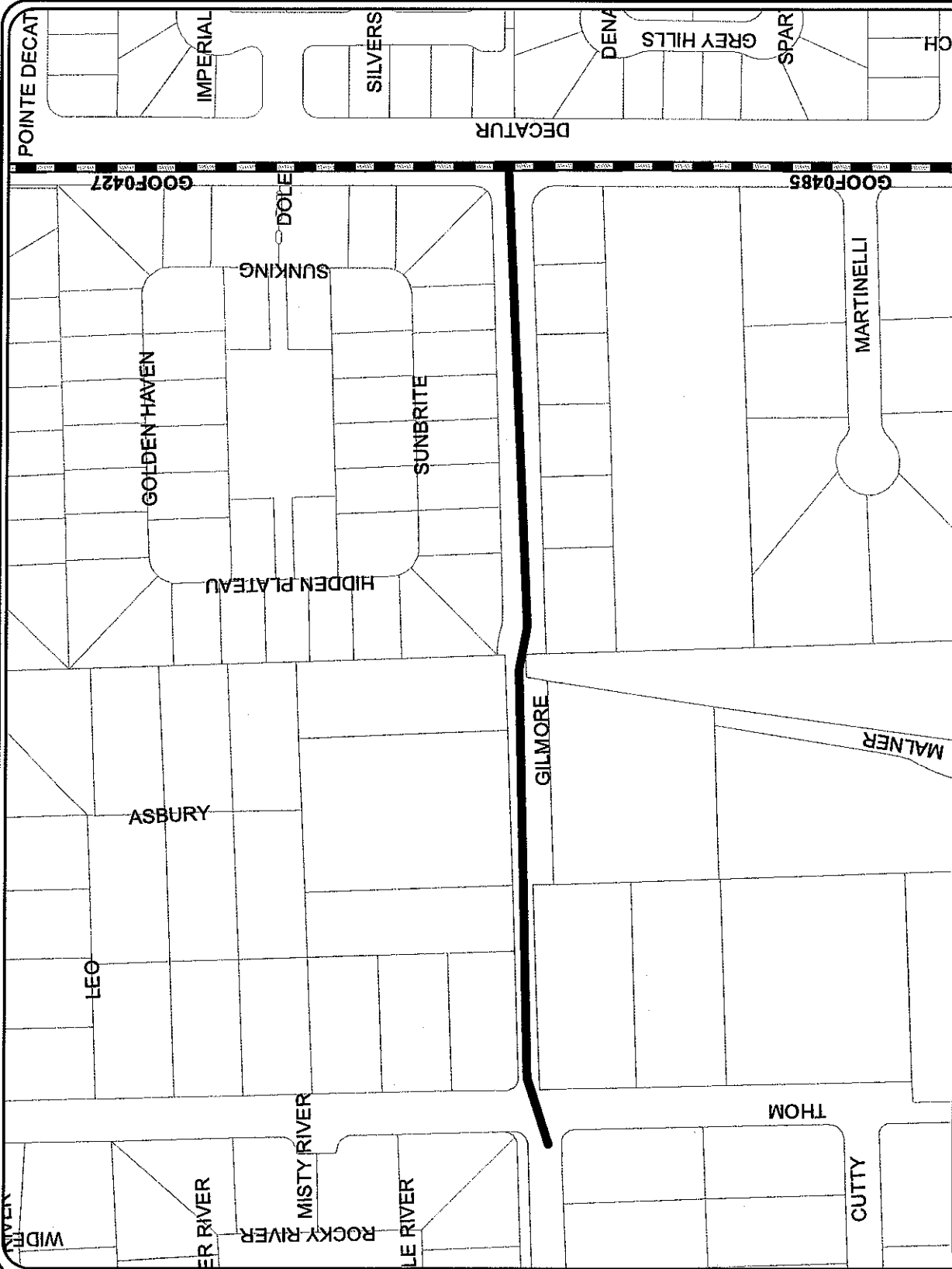
EXHIBIT A - GILMORE - THOM TO DECATUR - STORM DRAIN IMPROVEMENTS (LLDXXXX)
