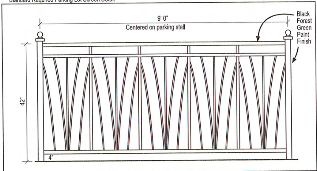
Standard Required Parking Lot Screen Detail
