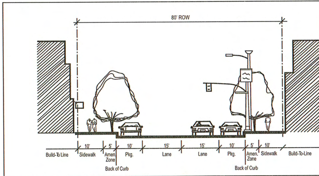
STREET SECTION
