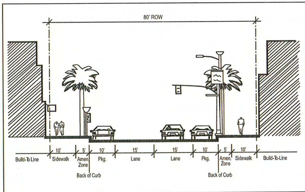
STREET SECTION
