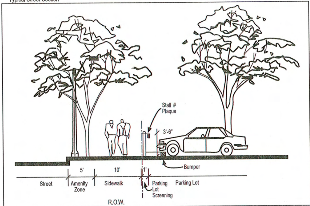
Typical Street Section
