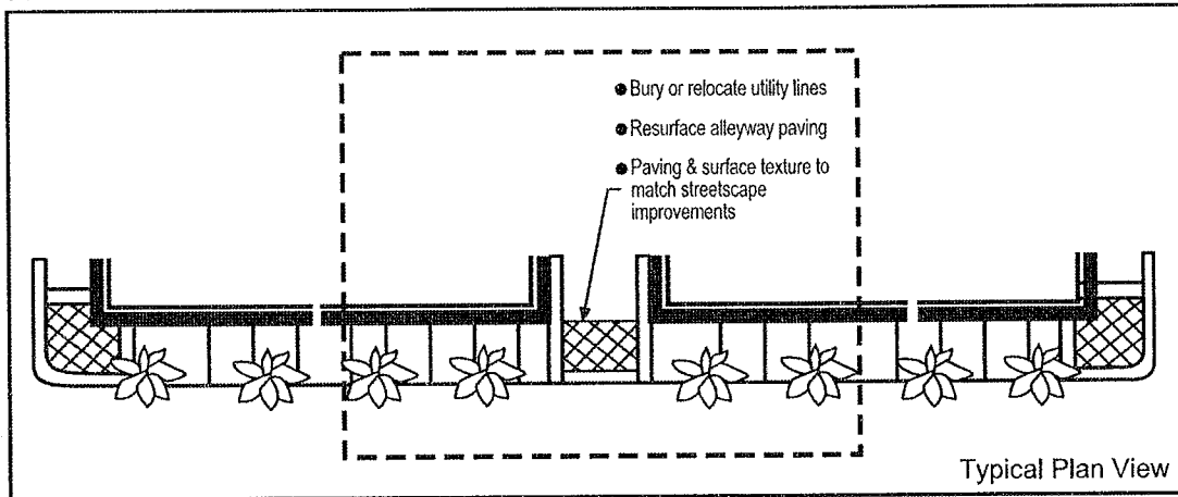
GRAPHIC 9: STANDARD REQUIRED ALLEYWAY TREATMENT.
