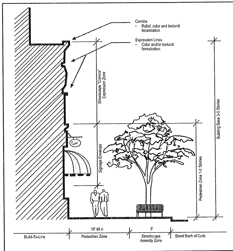
GRAPHIC 17: BUILDING FACADE AT STREET LEVEL
