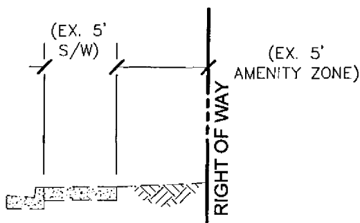
BONANZA RD. 105' R/W MAX, 100' TYPICAL (PUBLIC STREET) TYPICAL SECTION N.T.S.
