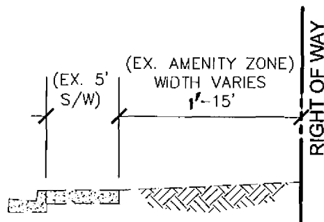
LAMB BLVD. 115' R/W MAX, 100' TYPICAL (PUBLIC STREET) TYPICAL SECTION N.T.S.
