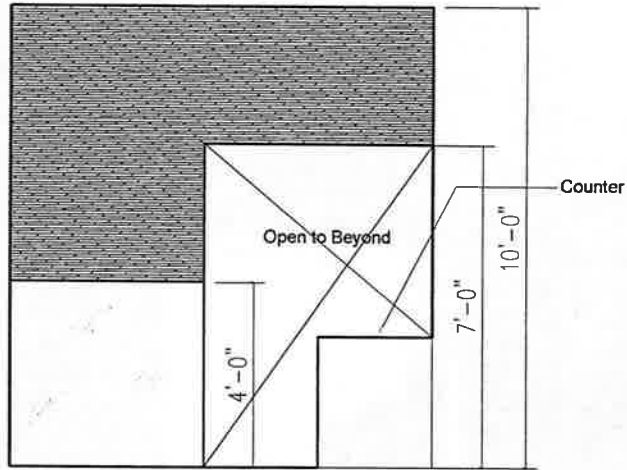
6.3 PREP ELEVATION
