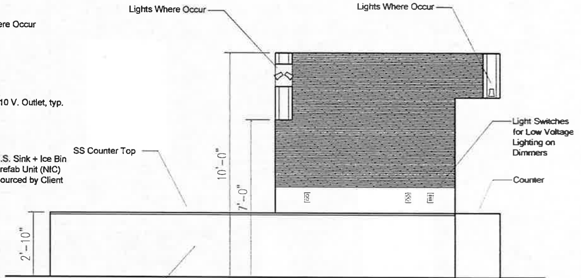
6.1 INTERIOR ELEVATION
