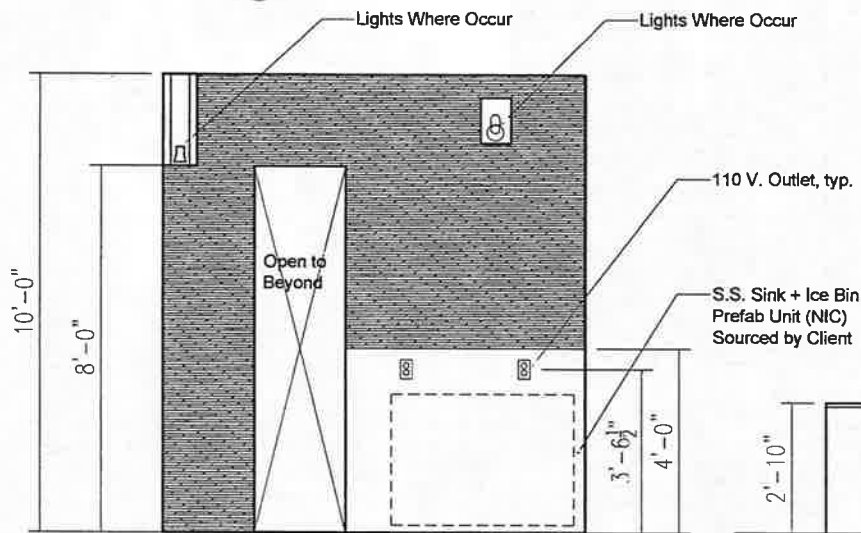
6.3 PREP ELEVATION
