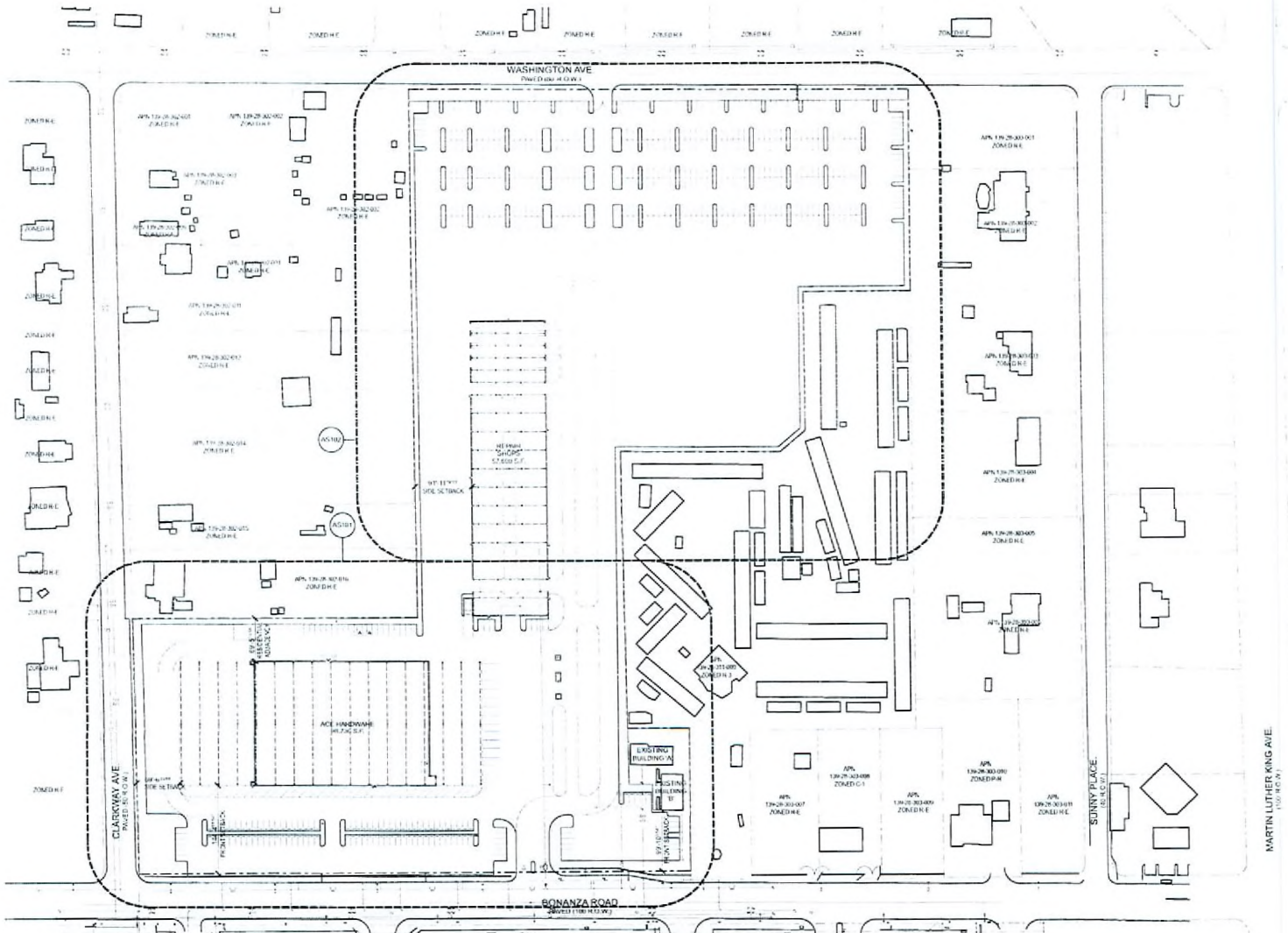
OVERALL SITE PLAN 1" = 80' 0"
