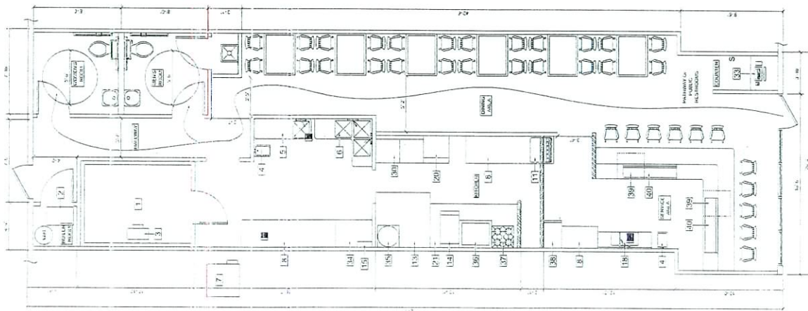
2 NEW FLOOR PLAN 1/4" = 1'-0"
