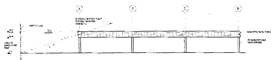
WEST ELEVATION
