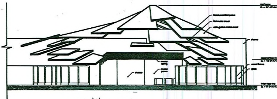
A1 east elevation 11-05-08 CC
