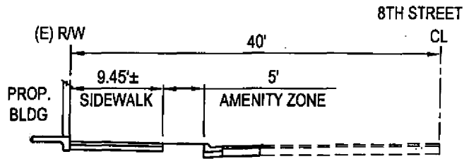
8TH STREET – TYPICAL SECTION (PUBLIC STREET – 80' R/W) NOT TO SCALE
