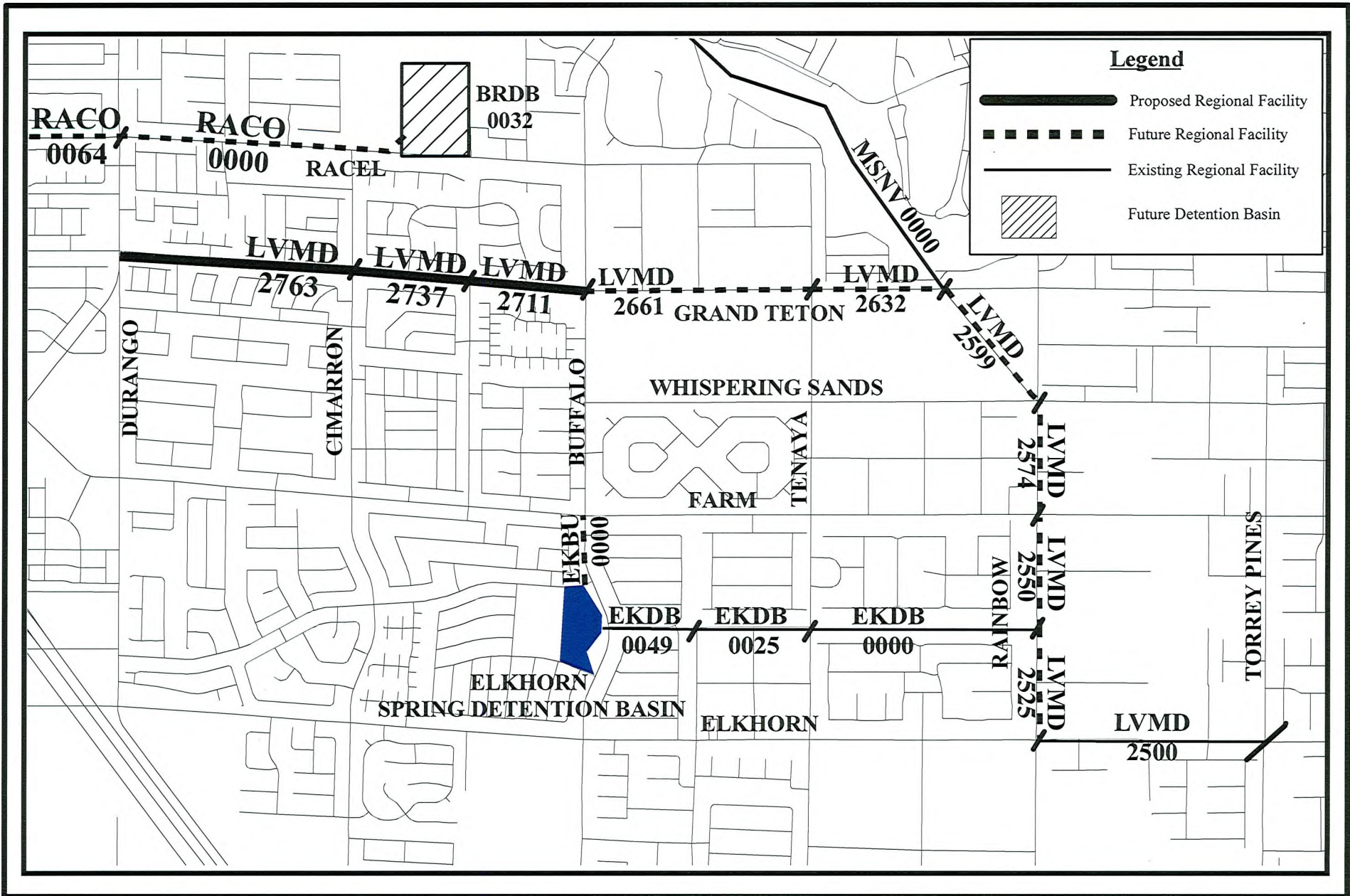
EXHIBIT A LAS VEGAS WASH - GRAND TETON, BUFFALO DRIVE TO DURANGO DRIVE (LAS22L08)
