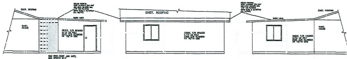
NORTH VIEW 2008 1/24/08
