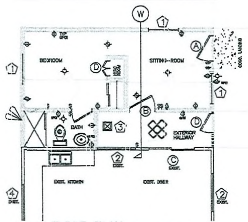
FLOOR PLAN 2008 1/24/08
