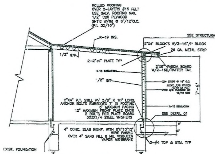
WALL SEC 'W' 2008 1/24/08
