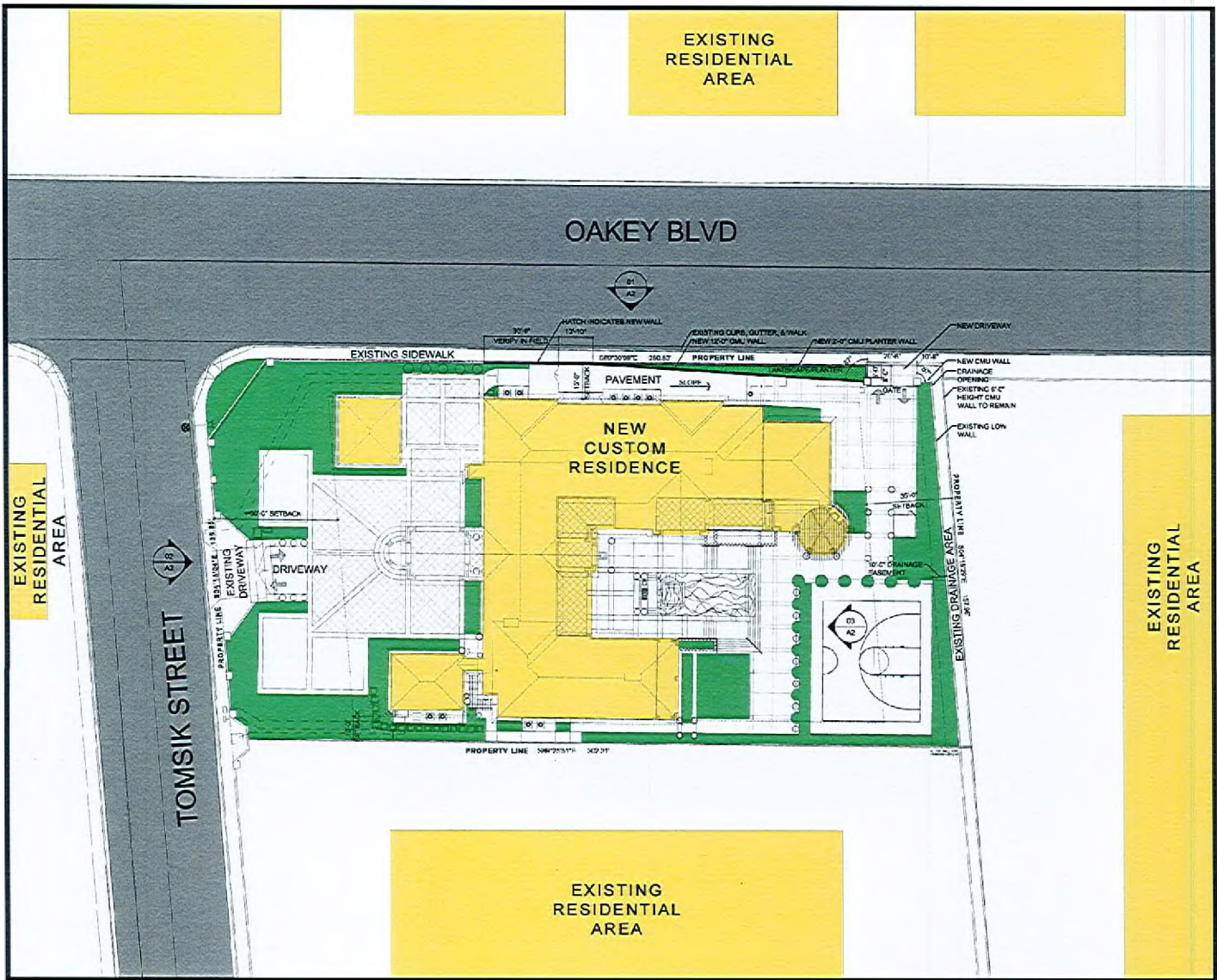
= 01 = SITE PLAN
