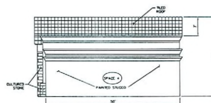
BUILDING 1 ELEVATION LOOKING WEST SCALE: 3/32" = 1'-0"
