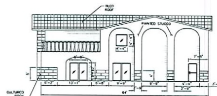
BUILDING 2 ELEVATION LOOKING SOUTH SCALE: 3/32" = 1'-0"
