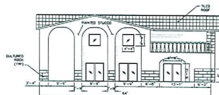
BUILDING 2 ELEVATION LOOKING NORTH SCALE: 3/32" = 1'-0"
