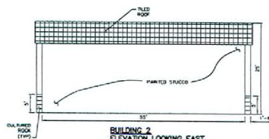
BUILDING 2 ELEVATION LOOKING EAST SCALE: 3/32" = 1'-0"
