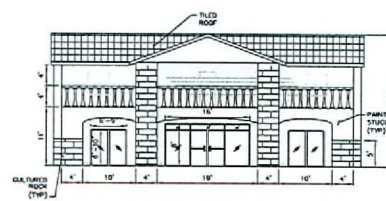
BUILDING 2 ELEVATION LOOKING WEST SCALE: 3/32" = 1'-0"
