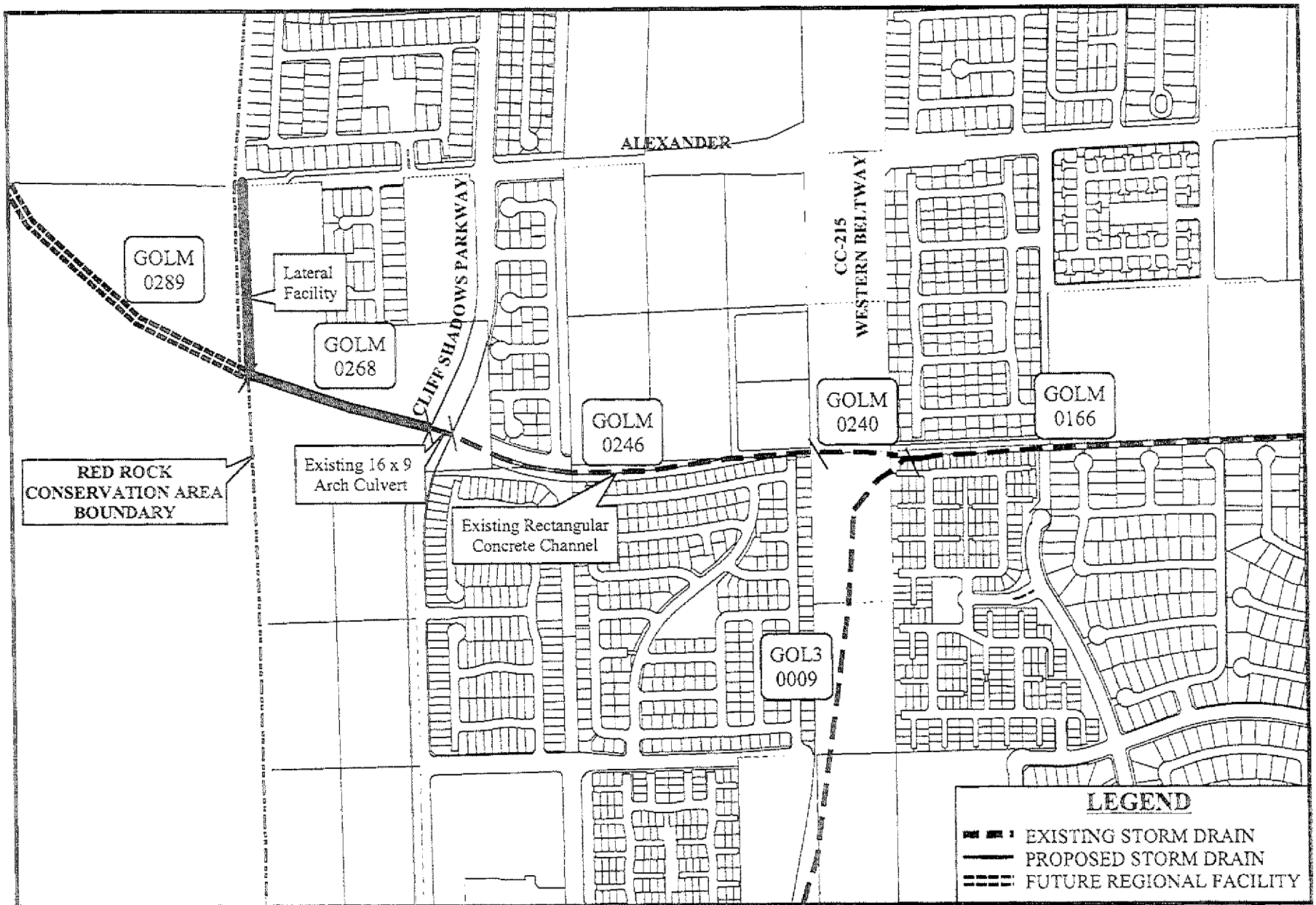
EXHIBIT A GOWAN LONE MOUNTAIN SYSTEM (LAS.10.Y.05) (GILMORE CLIFF SHADOWS PARK ARCH CULVERT EXTENSION)
