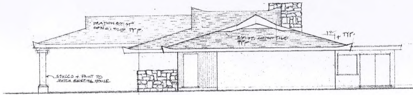
EAST ELEVATION 1/4"=1'-0"
