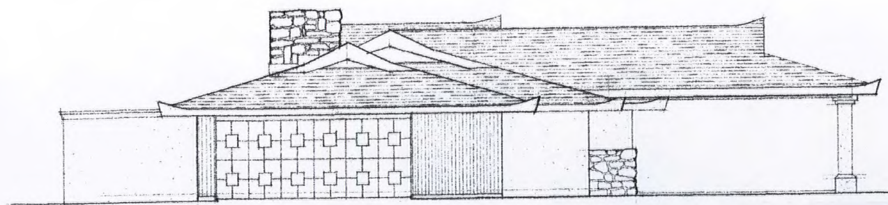
WEST (BIRCH STREET) ELEVATION 1/4"=1'-0"
