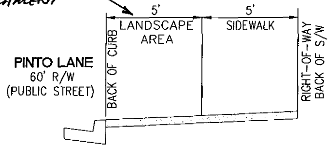
TYPICAL SECTION NO SCALE
