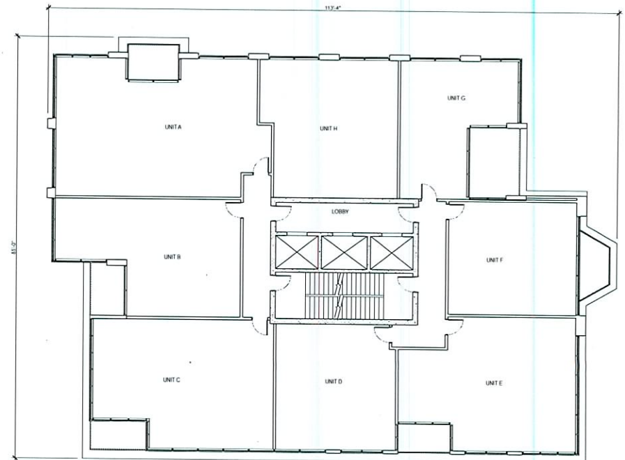
TYPICAL FLOORPLATE 31-50
